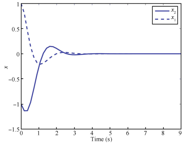
Fig. 1 Responses of state x with p(t) = 0
